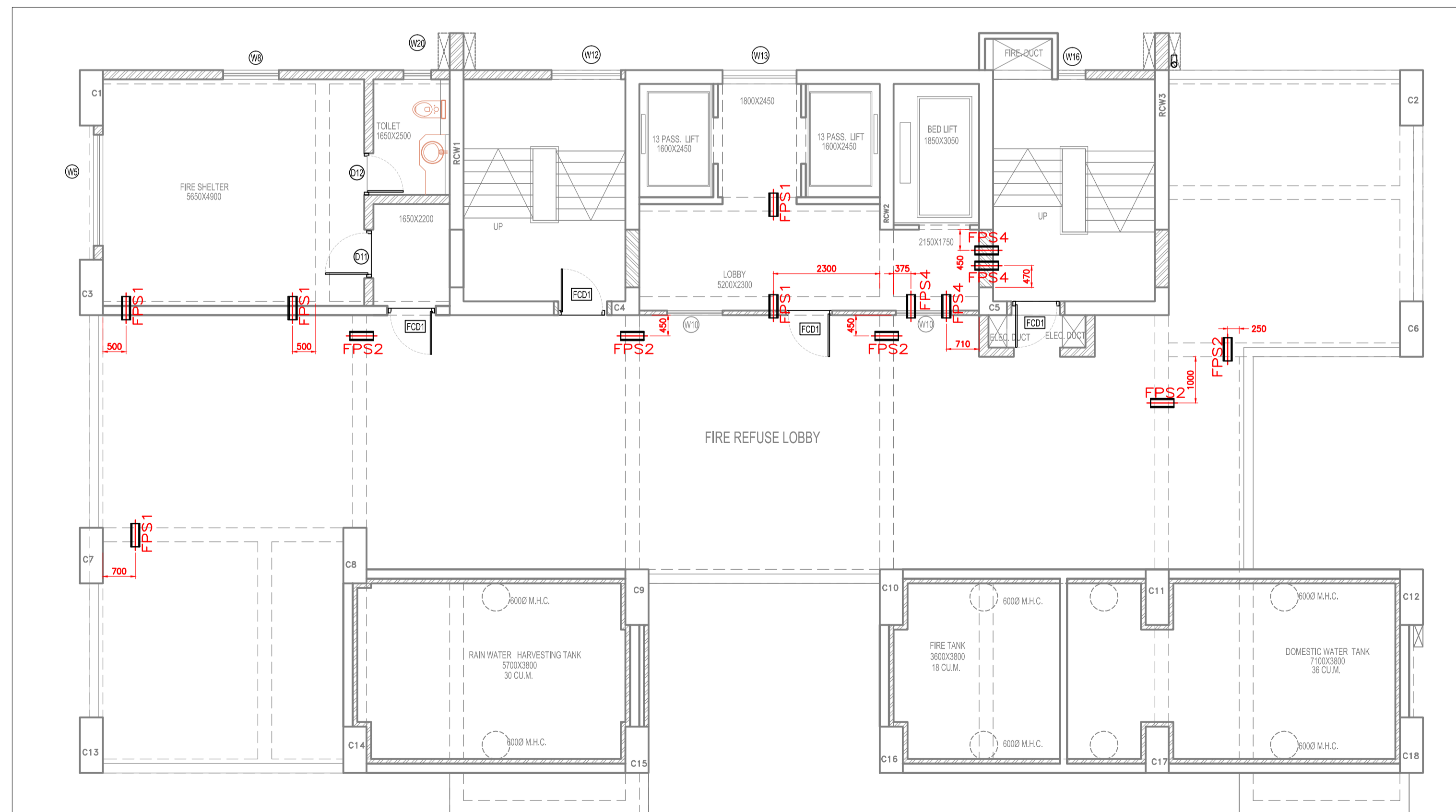
PIPE SLEEVES FOR FIRE PIPE SCALE 1:75
